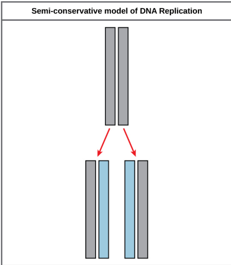
Figure 2. The semiconservative model of DNA replication is shown. Gray indicates the original DNA strands, and blue indicates newly synthesized DNA.
