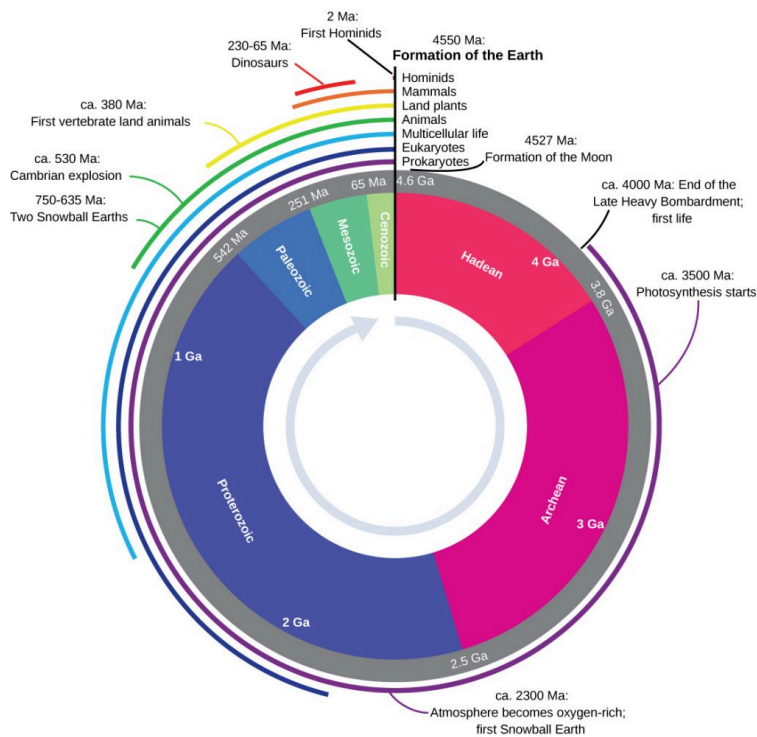
Figure 1. Geological Time Clock
