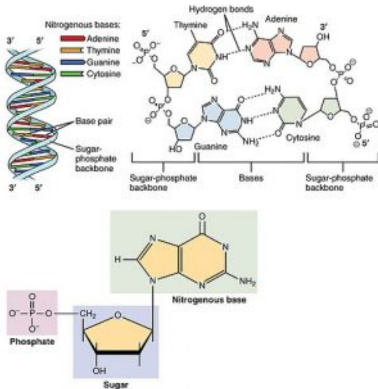
Figure 1. Basic DNA structure.
