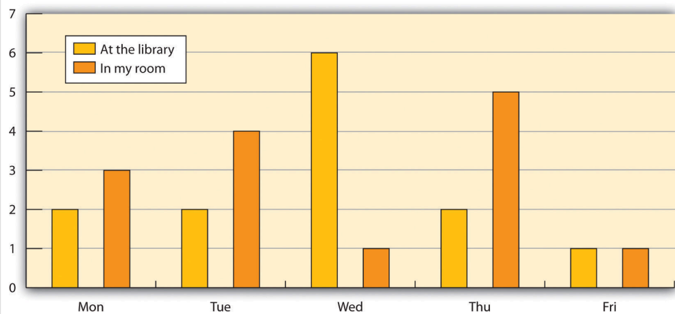
Figure 5.4 Bar Chart
