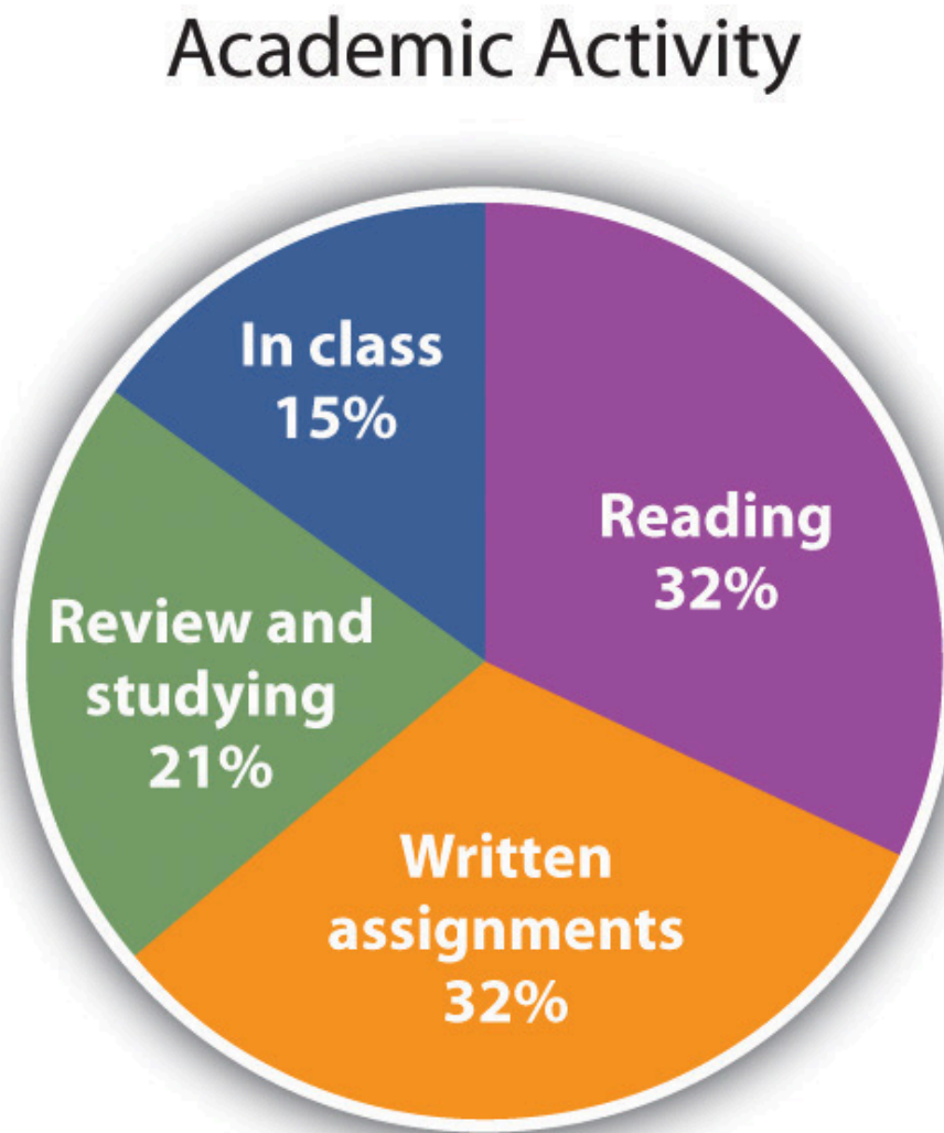
Figure 5.6 Pie Chart
