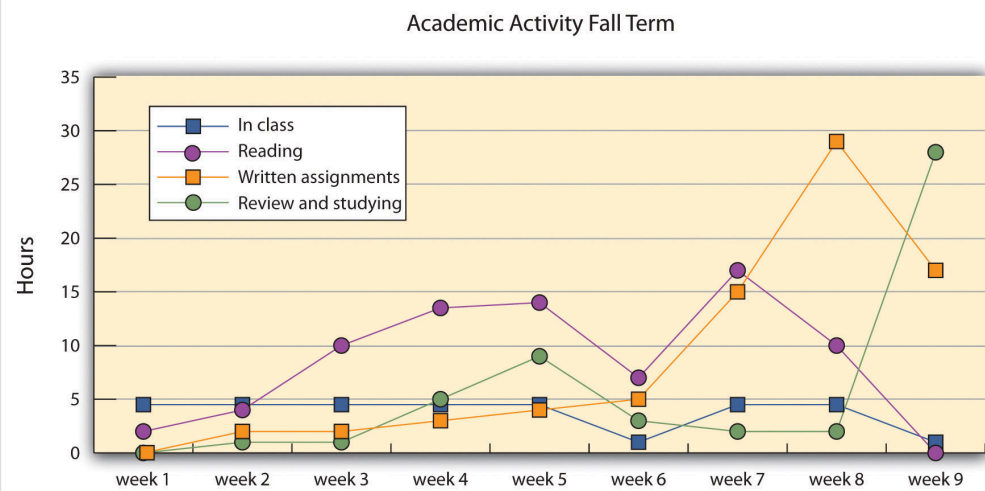
Figure 5.5 Line Chart
